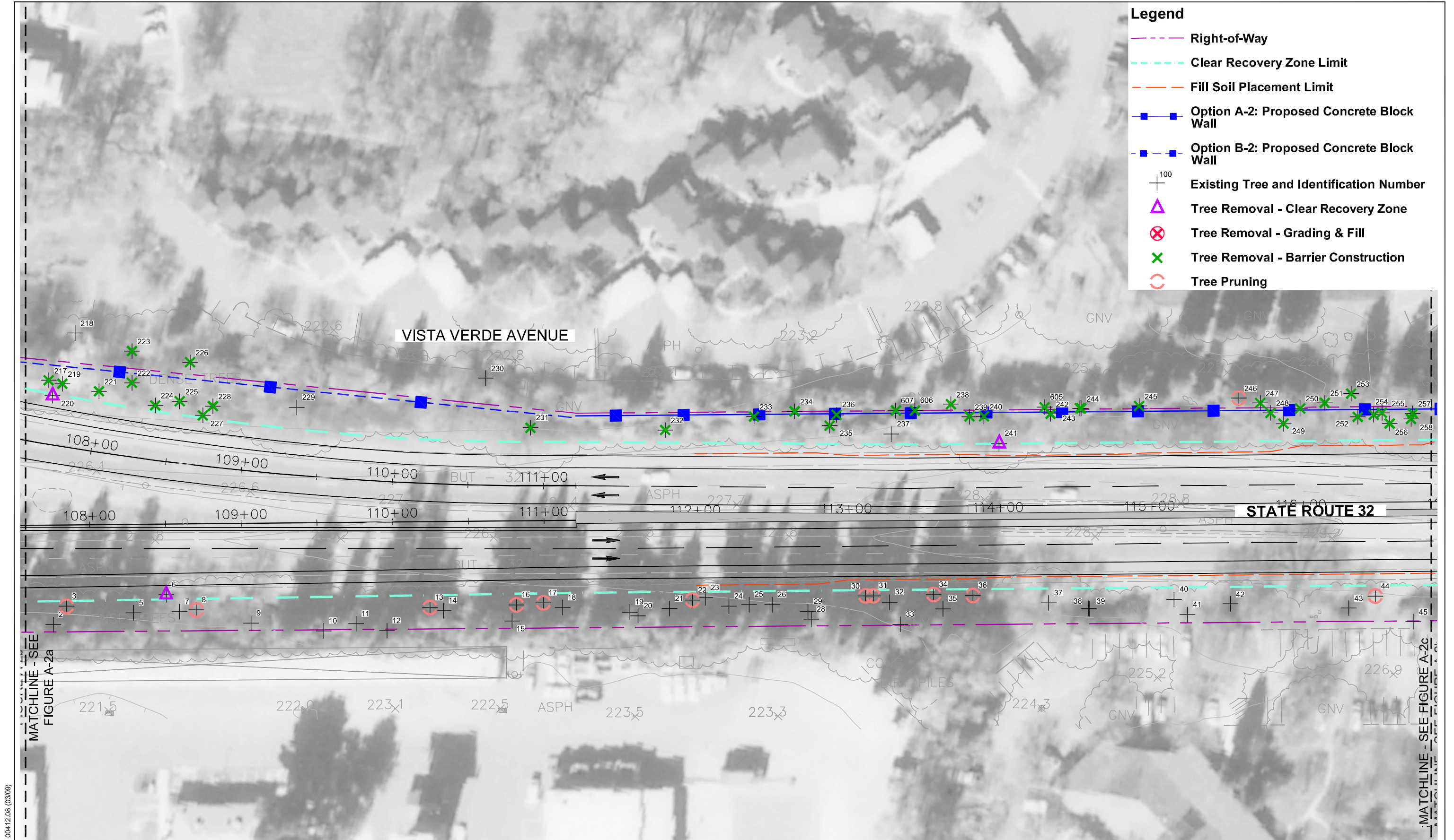
Figure A-2b SR 32 Widening Arborist Report - Concrete Block Wall
