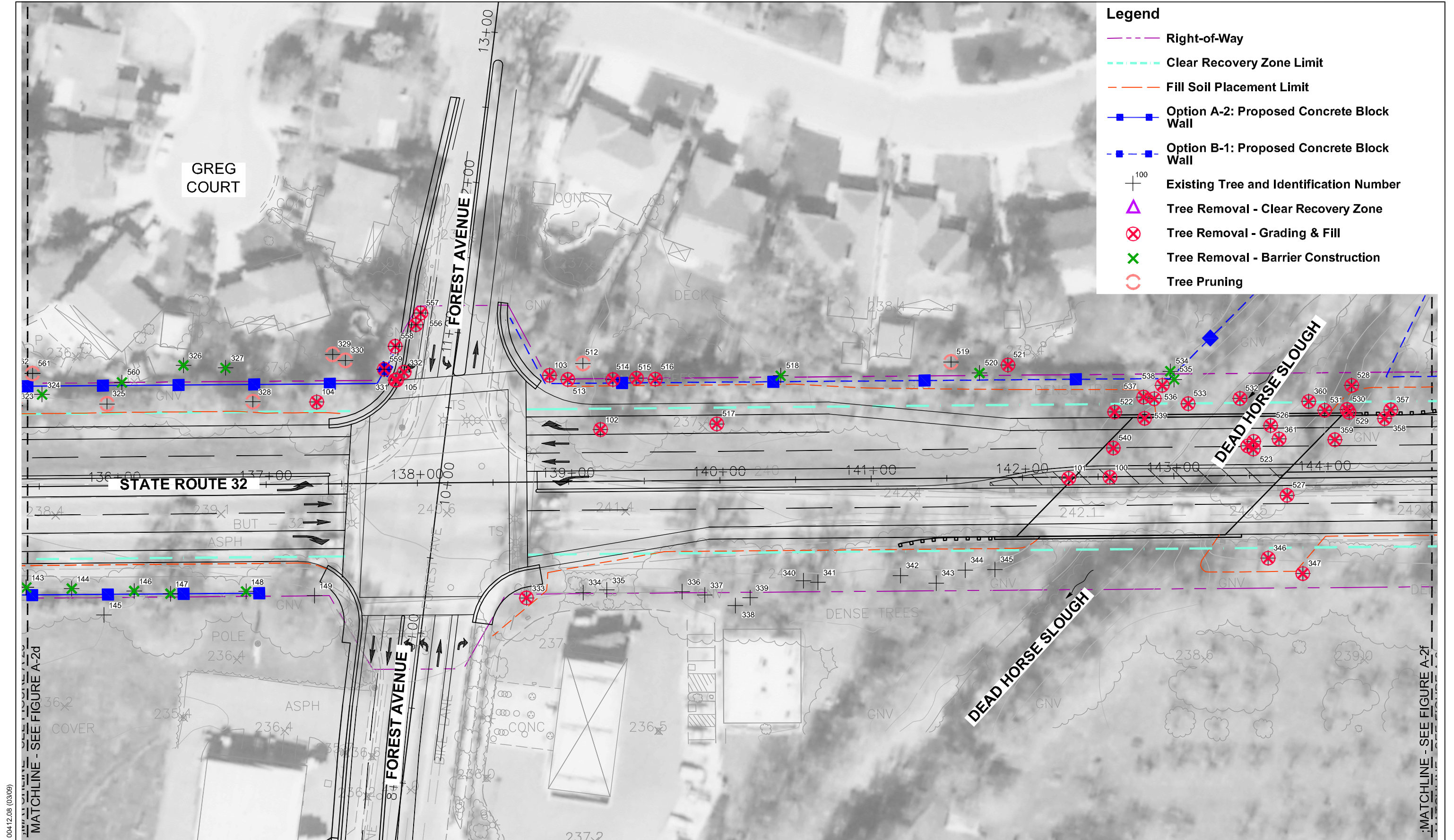
Figure A-2e SR 32 Widening Arborist Report - Concrete Block Wall
